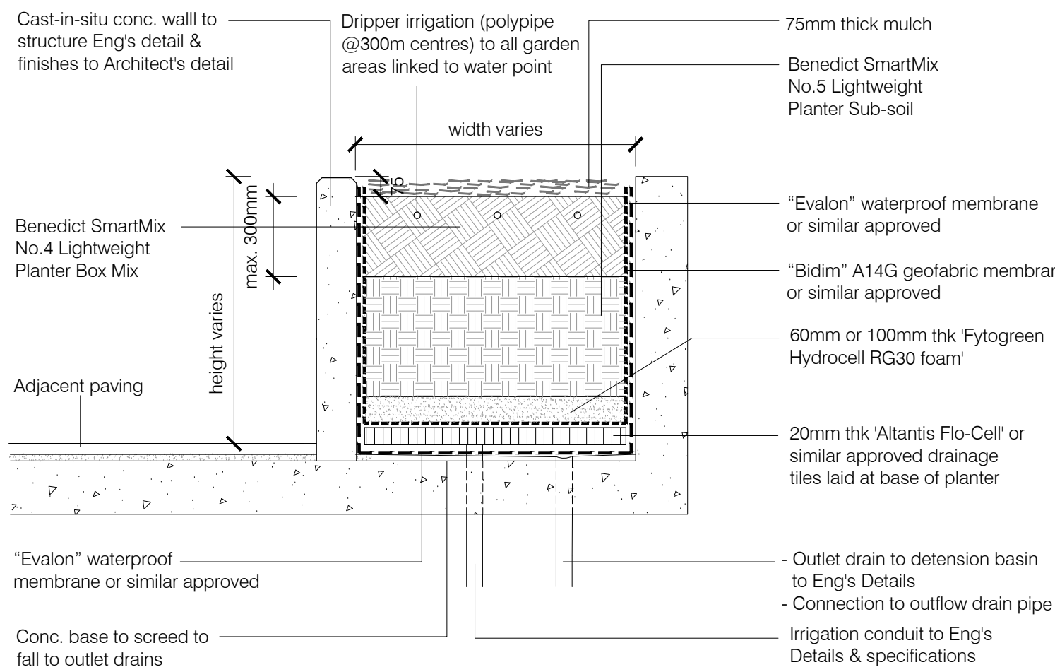
TYPICAL DETAIL 01: on-structure planter
