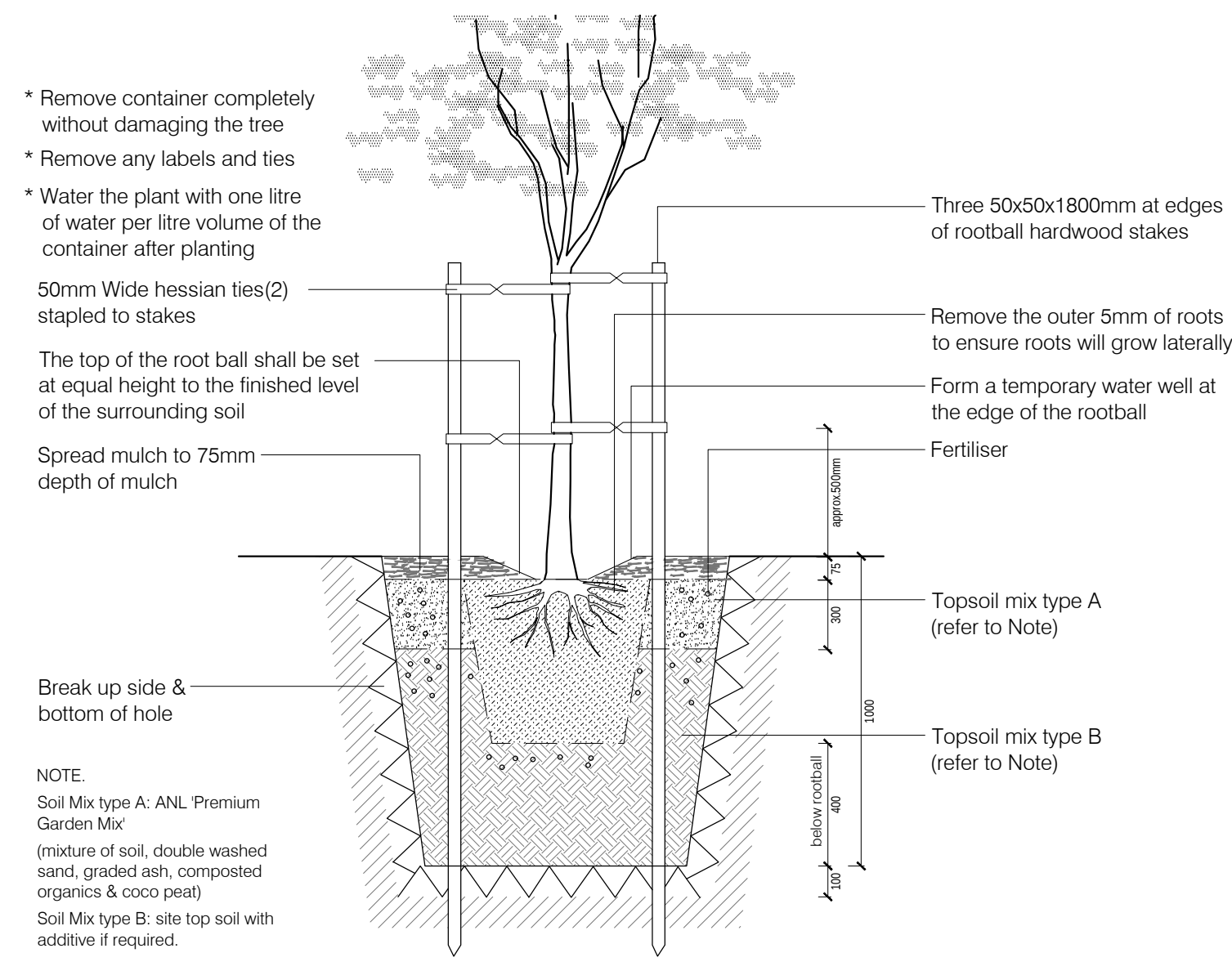
TYPICAL DETAIL 04: tree planting (on-site)
