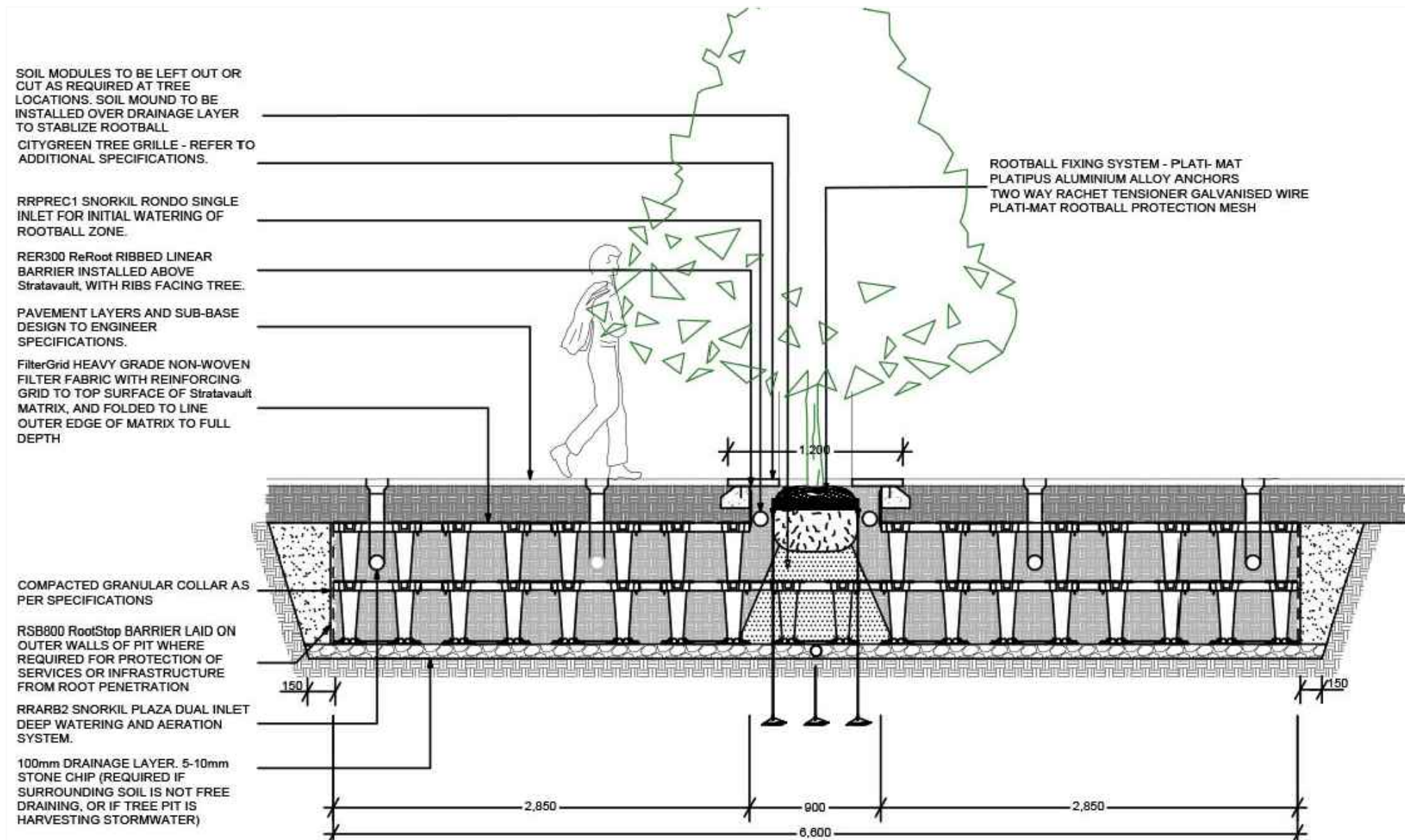
TYPICAL DETAIL 05: stratavault system by city green
