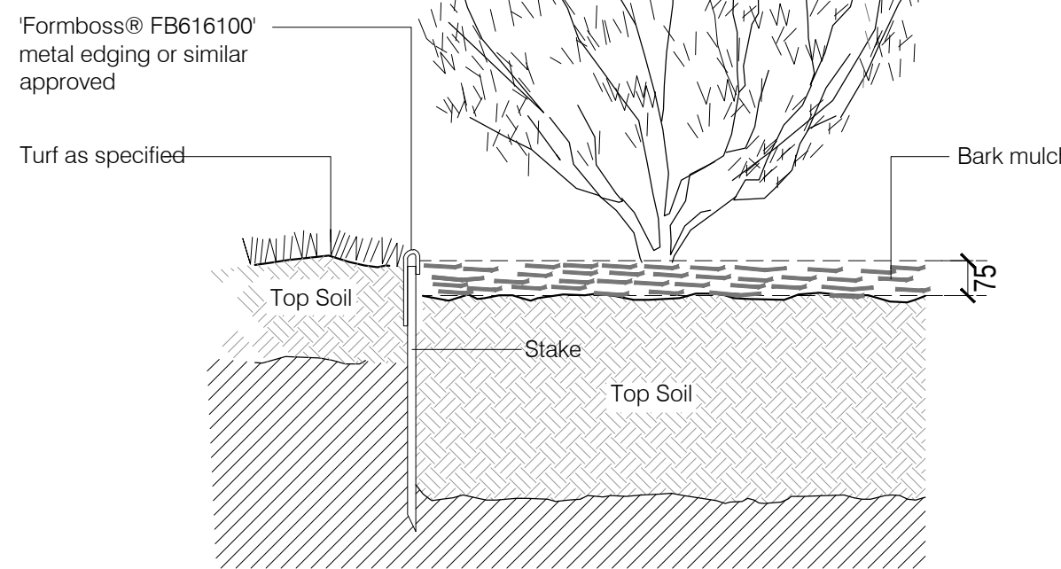
TYPICAL DETAIL 03: metal edging
