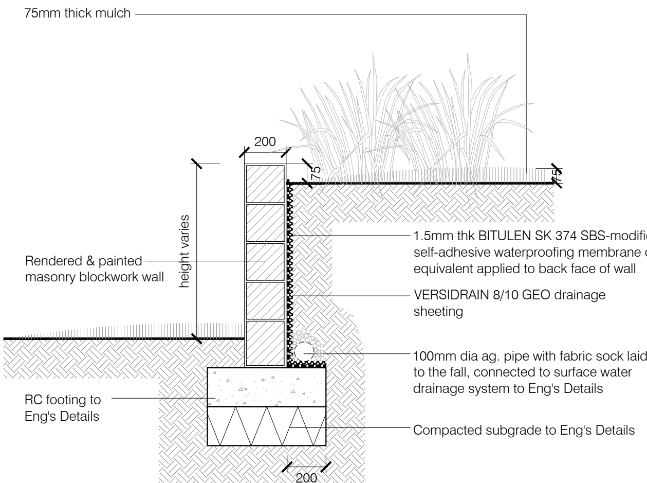
TYPICAL DETAIL 02: retaining wall
